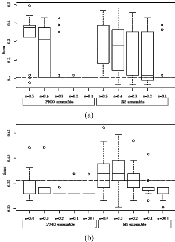
Figure 1. Boxplots of the errors with DNA microarray data. Single hierarchical clustering, PMO and RS ensembles with different 1 + e distortions are compared, using 30 replications for each experiment, and 50 clusterings for each ensemble. The thin lines inside the boxes represent the median value. The error achieved with single hierarchical clustering is represented by the horizontal dash-dotted line. (a) DLBCL-FL data set (b) Primary-Metastasis DNA microarray data.
