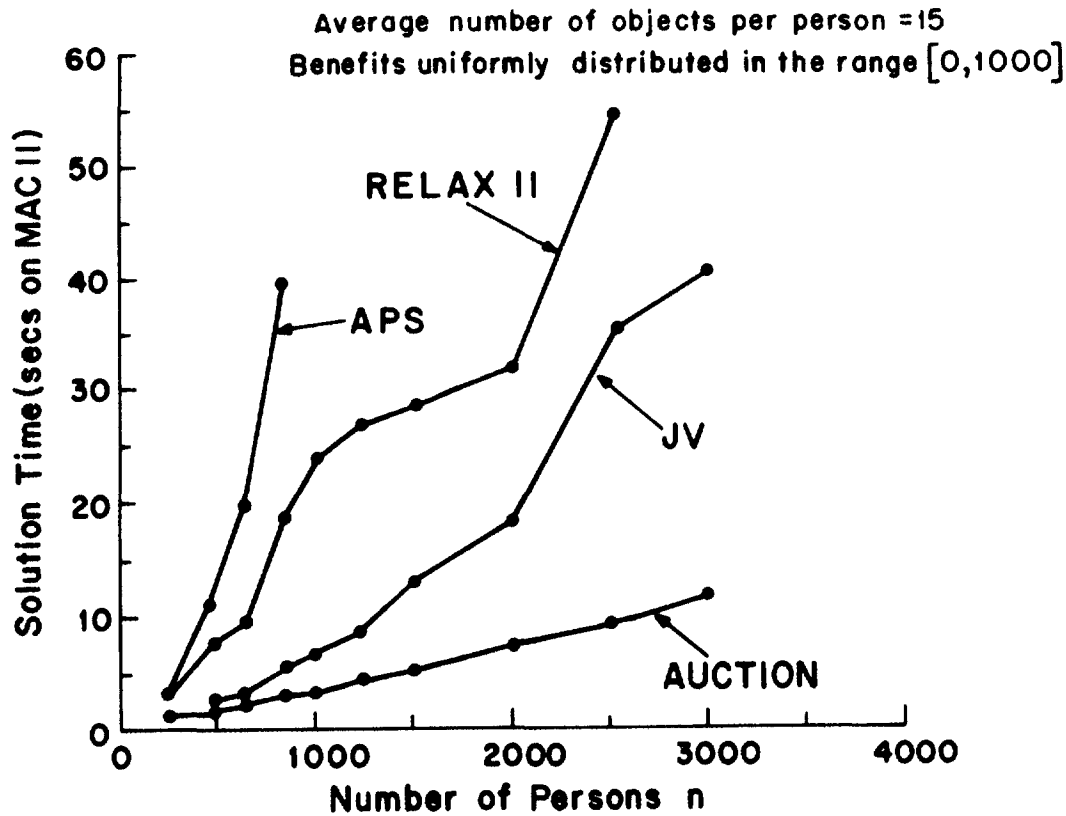
Figure 7: Computational results comparing various codes using a MAC-II on randomly generated problems. For all test problems, the number of feasible assignment pairs is 15n , where n is the number of persons, and the benefits a_{ij} are integers chosen according to a uniform distribution from the range [0, 1000] .
