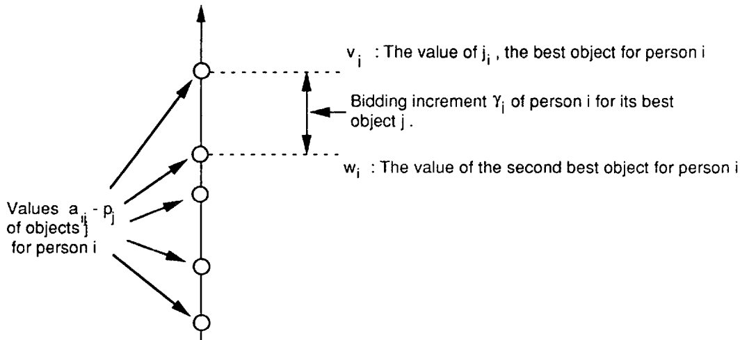
Figure 1: In the naive auction algorithm, even after the price of j_i is increased by the bidding increment \gamma_i , j_i continues to be the preferred object, so the bidder i is happy following the round. However, \gamma_i = 0 if there are two objects most preferred by the bidder i .
