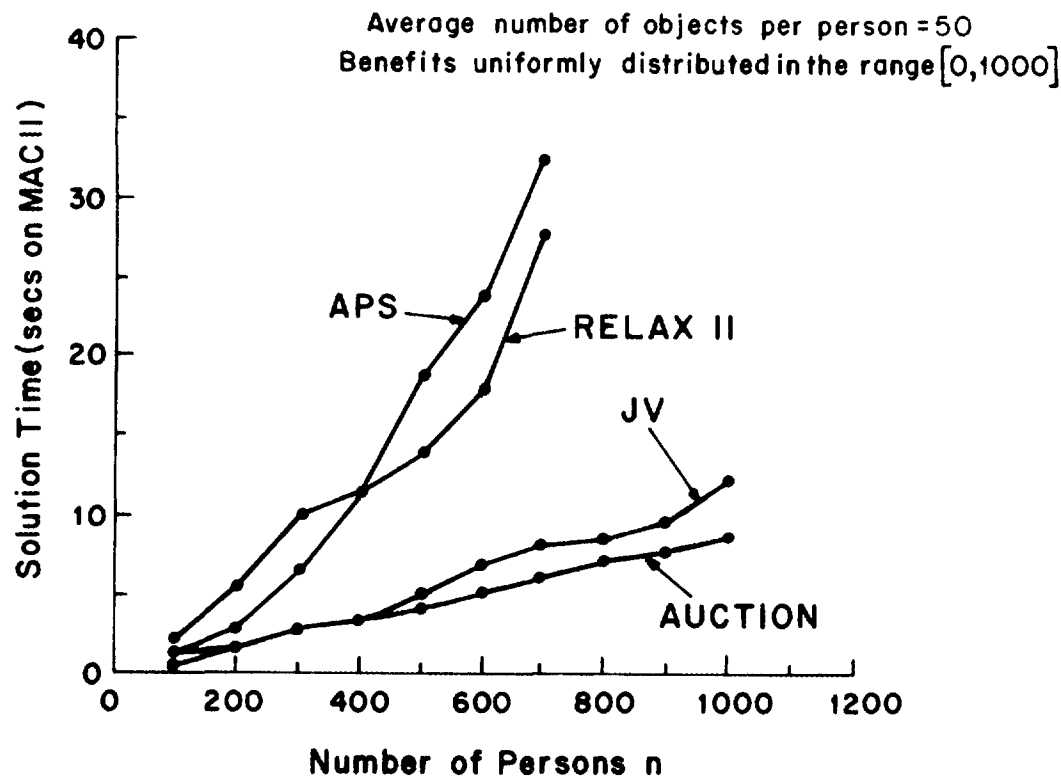
Figure 8: Computational results comparing various codes using a MAC-II on randomly generated problems. For all test problems, the number of feasible assignment pairs is 50n , where n is the number of persons, and the benefits a_{ij} are integers chosen according to a uniform distribution from the range [0, 1000] .
