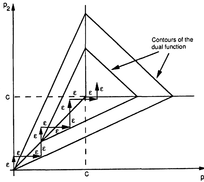
Figure 5: Illustration of the sequence of prices generated by the auction algorithm for the example of Figure 4, in relation to the contours of the dual function
