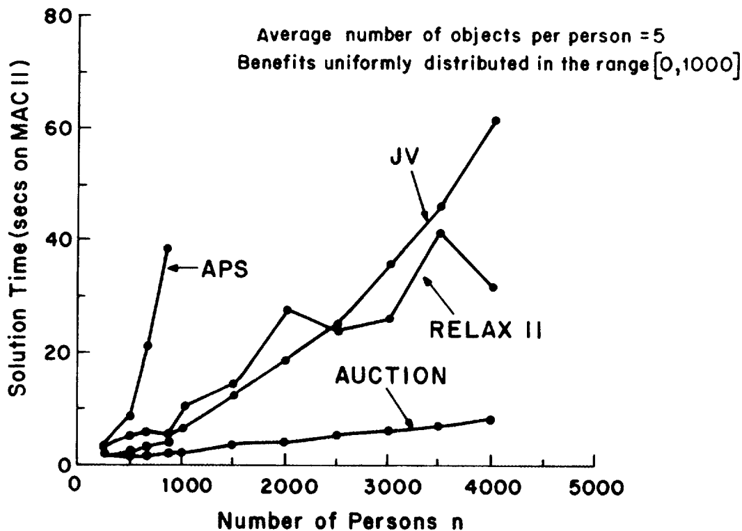
Figure 6: Computational results comparing various codes using a MAC-II on randomly generated problems. For all test problems, the number of feasible assignment pairs is 5n , where n is the number of persons, and the benefits a_{ij} are integers chosen according to a uniform distribution from the range [0, 1000] .
