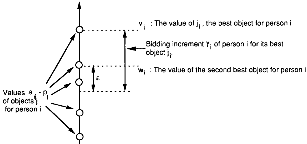
Figure 3: In the auction algorithm, even after the price of the preferred object j_i is increased by the bidding increment \gamma_i , j_i will be within \epsilon from being most preferred, so the bidder i is almost happy following the round.
