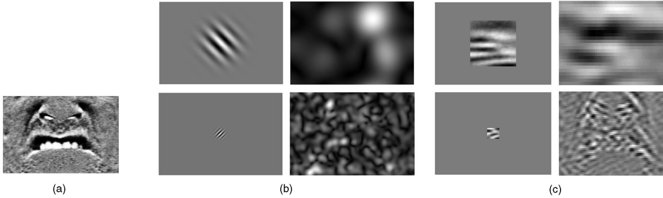
Fig. 10. (a) Original \delta -image. (b) Gabor kernels (low and high frequency) with the magnitude of the filtered image to the right. (c) Local PCA kernels (large and small scale) with the corresponding filtered image.
