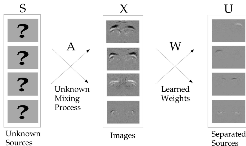
Fig. 7. Image synthesis model for the ICA representation.
