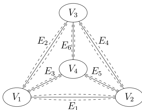
Figure 1: Edges in the figure represent sets of edges of G having endpoints in distinct V_i 's.
