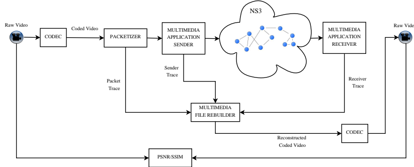
Figure 1: The proposed evaluation framework.
