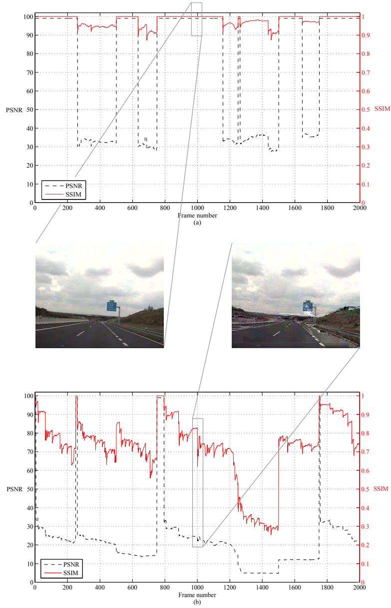
Figure 3: PSNR and SSIM - Scenario 1 for PER = 0.001 and PER = 0.01 .
