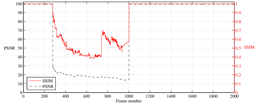
Figure 5: PSNR and SSIM - Scenario 2 with UDP cross-traffic.
