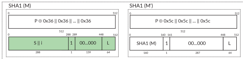
Fig. 5. Precomputing a specific word-expansion
