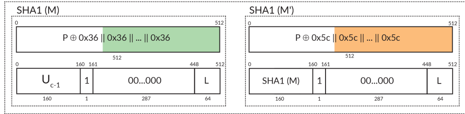
Fig. 4. Constant-padding scheme
