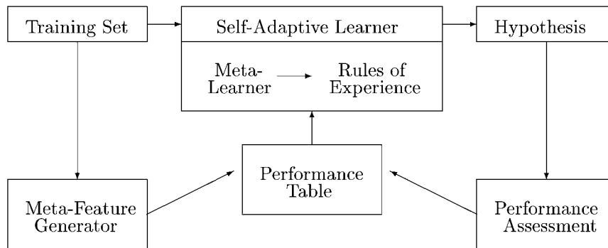
Figure 2. A flow diagram of a self-adaptive learner.
